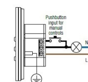
WITH MECHANICAL PUSHBUTTON CONNECTED TO THE LOAD
