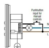
WITH MECHANICAL PUSHBUTTON CONNECTED TO THE POWER SUPPLY
